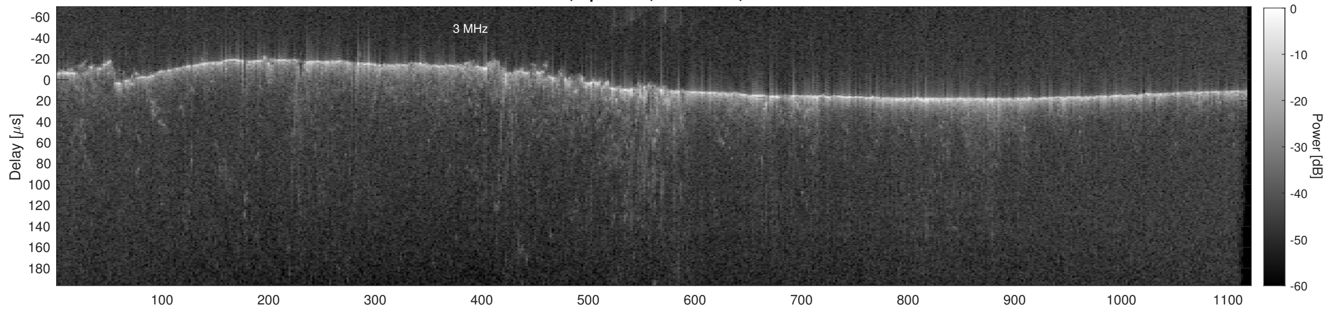
Orbit 22818, Cluttergram
