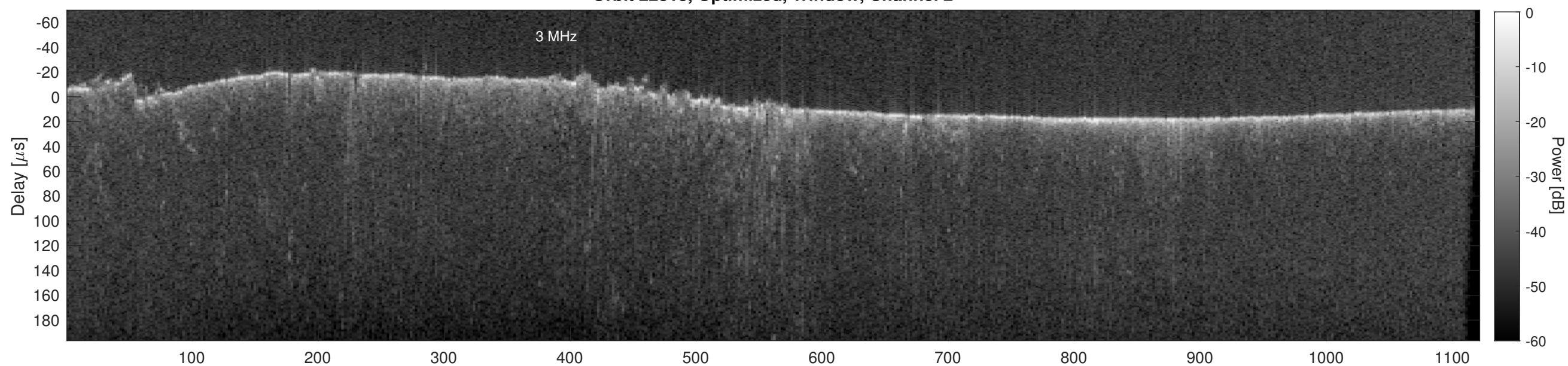
Orbit 22818, Cluttergram
