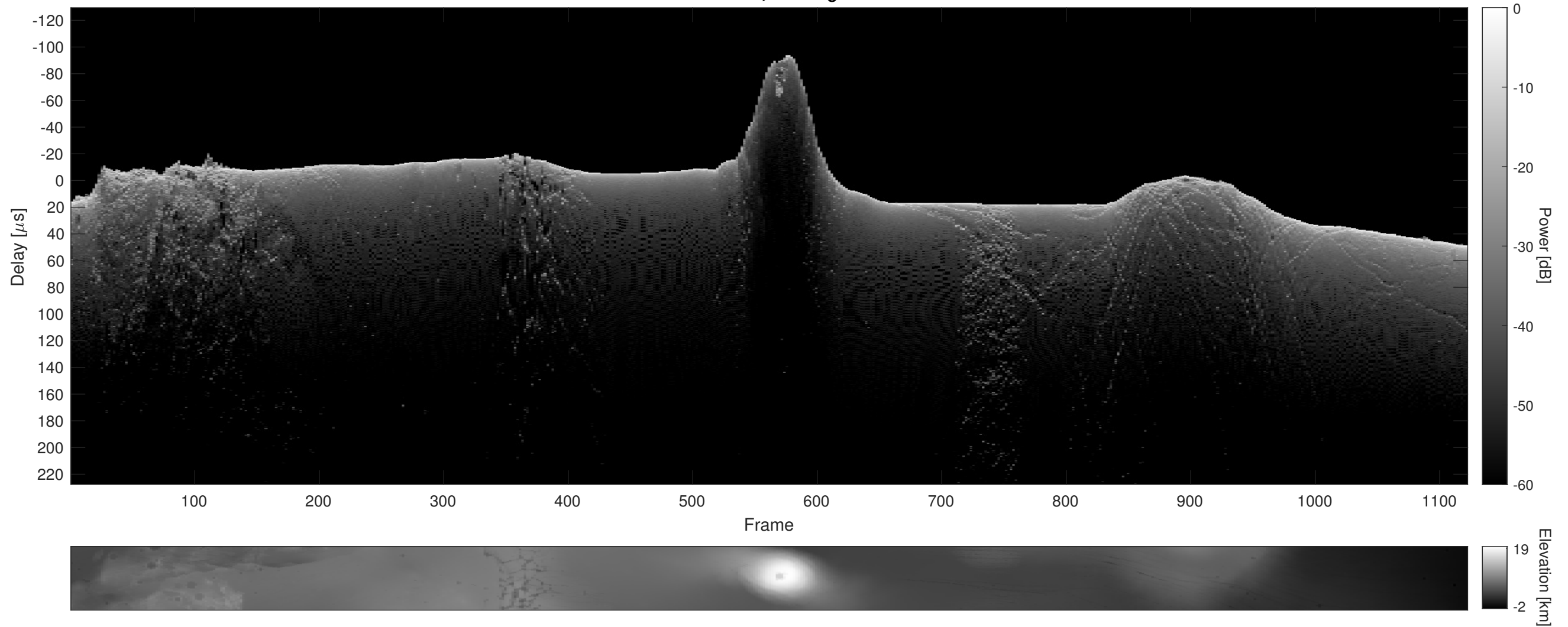
Orbit 22820, Cluttergram
