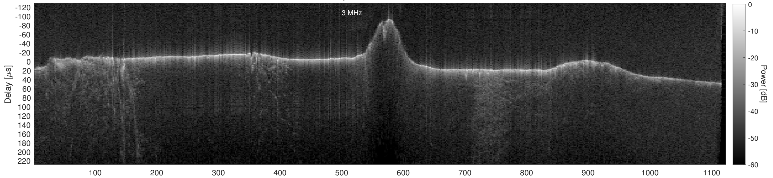
Orbit 22820, Cluttergram
