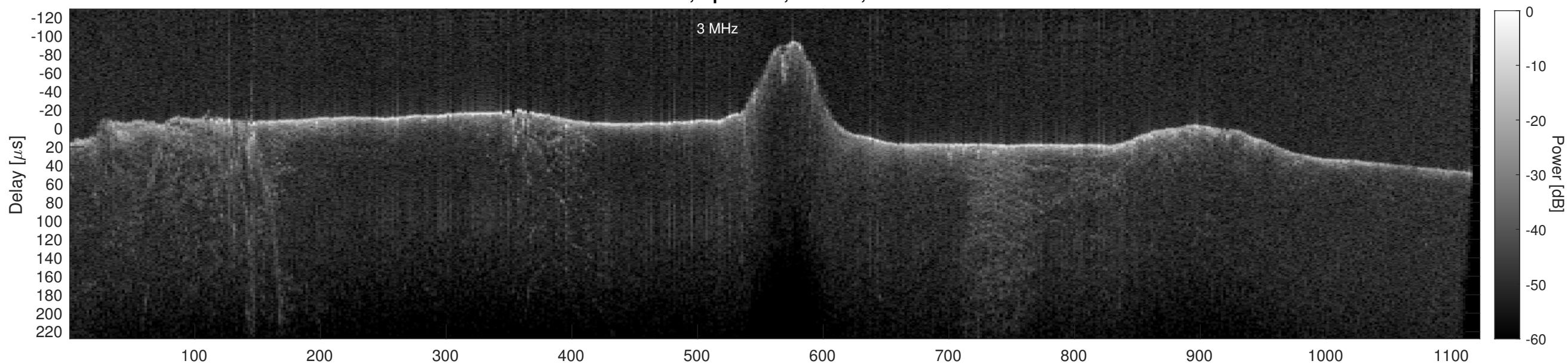
Orbit 22820, Cluttergram
