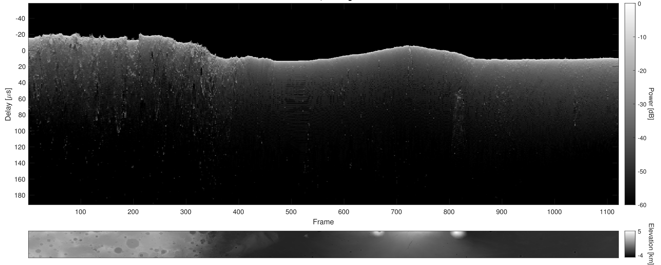
Orbit 22821, Cluttergram
