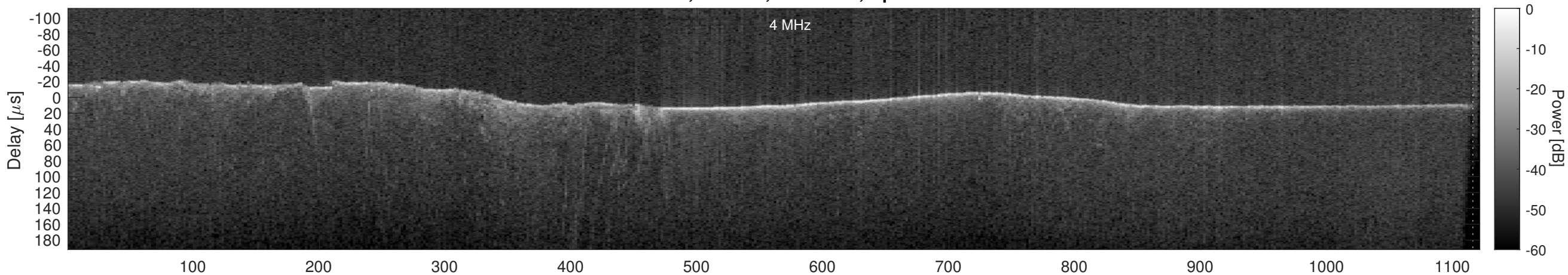
Orbit 22821, Cluttergram
