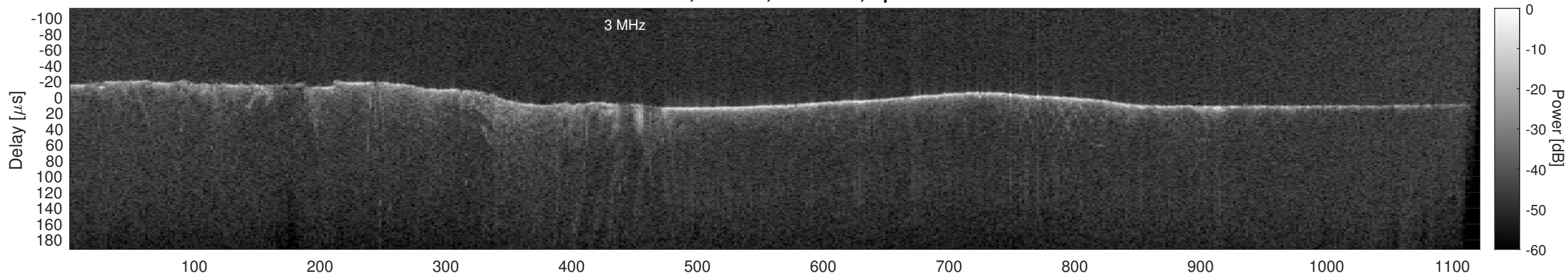
Orbit 22821, Cluttergram
