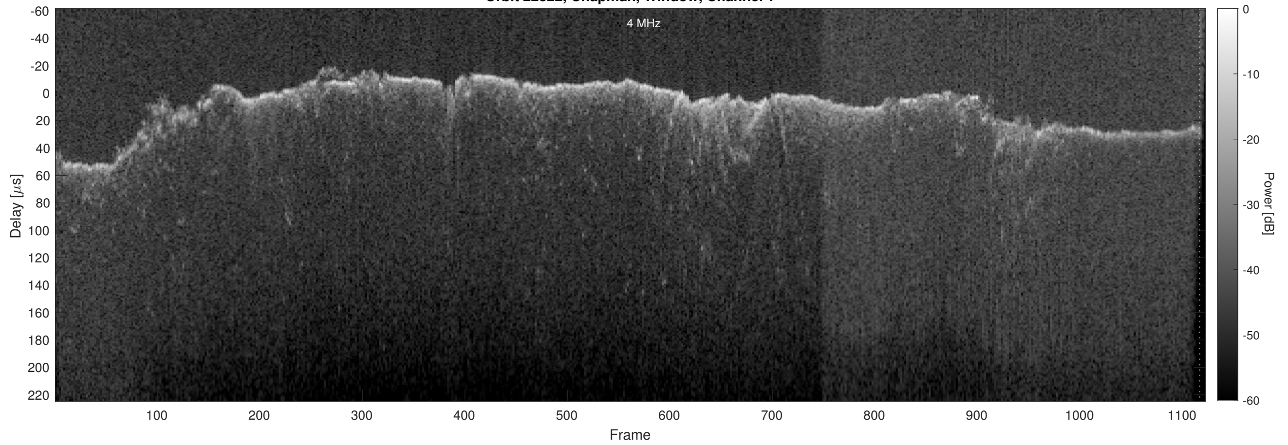
Orbit 22822, Chapman, Window, Channel 2
