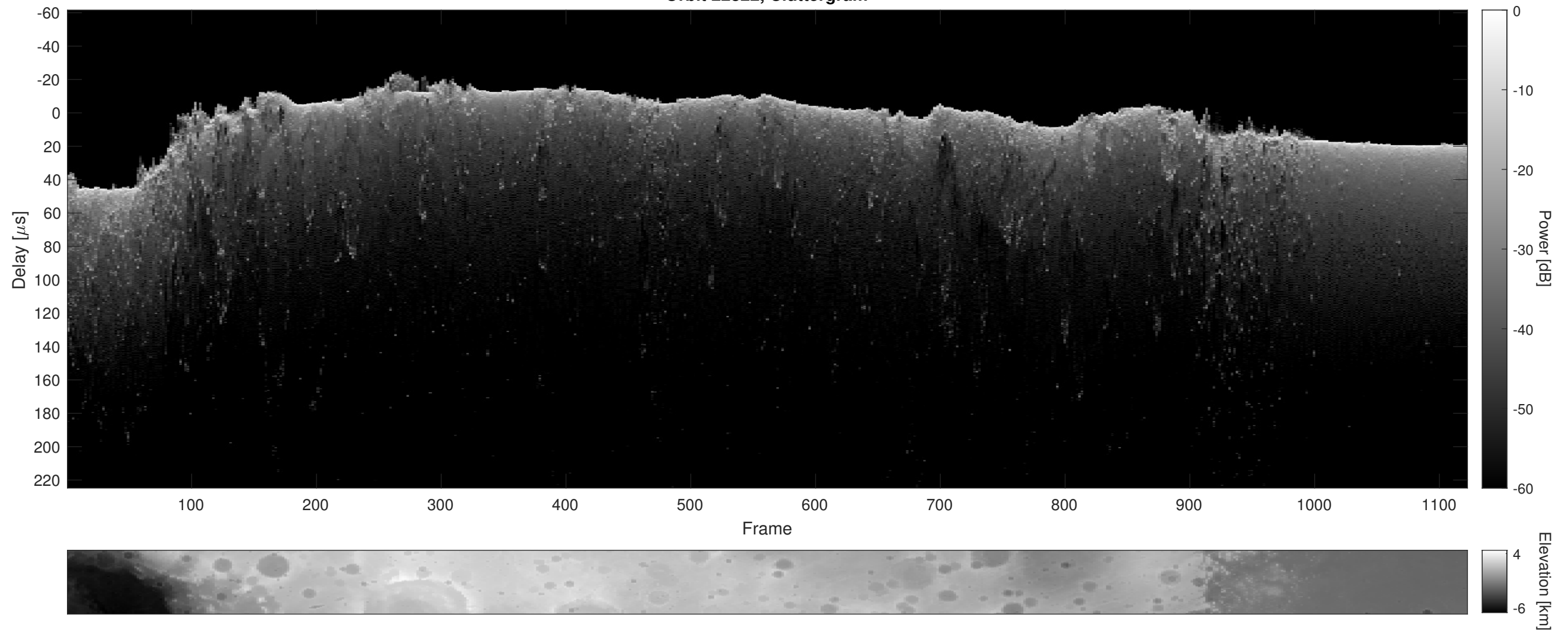
Orbit 22822, Cluttergram
