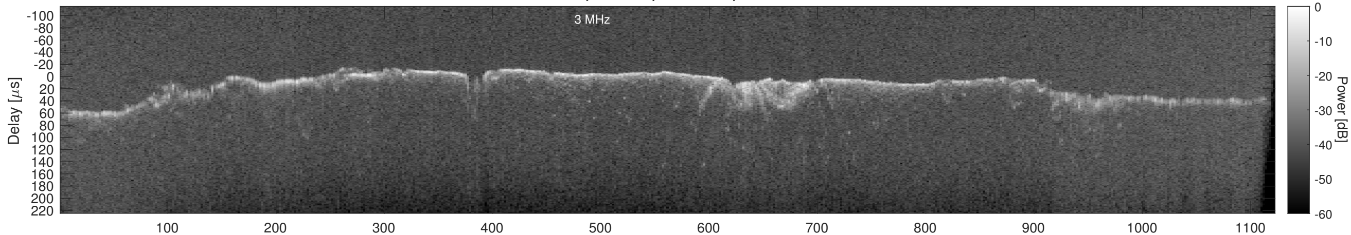
Orbit 22822, Window, Channel 2, Chapman
