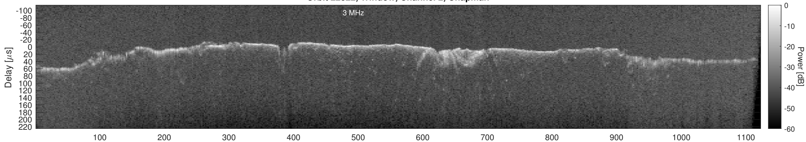
Orbit 22822, Window, Channel 2, Optimized
