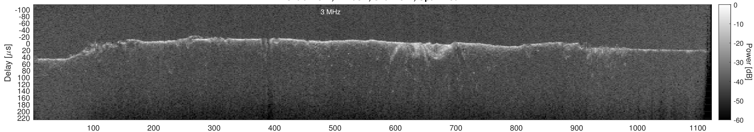
Orbit 22822, Cluttergram
