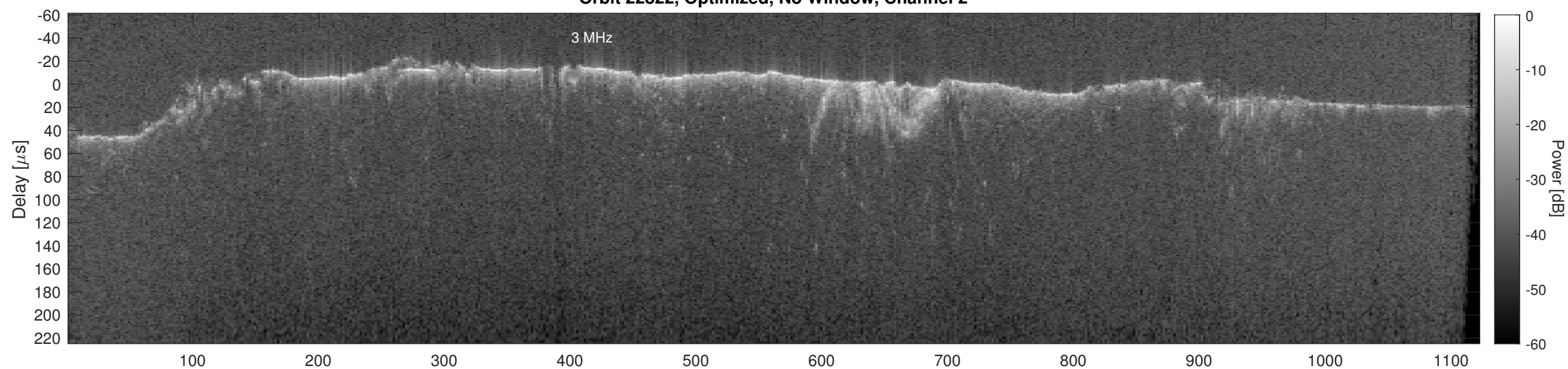
Orbit 22822, Cluttergram
