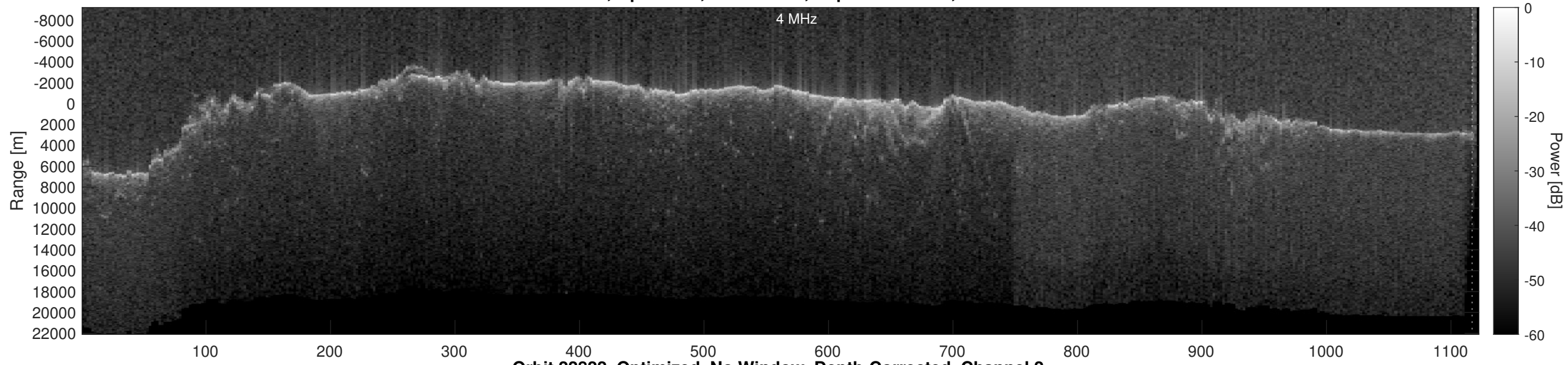
Orbit 22822, Optimized, No Window, Depth-Corrected, Channel 2
