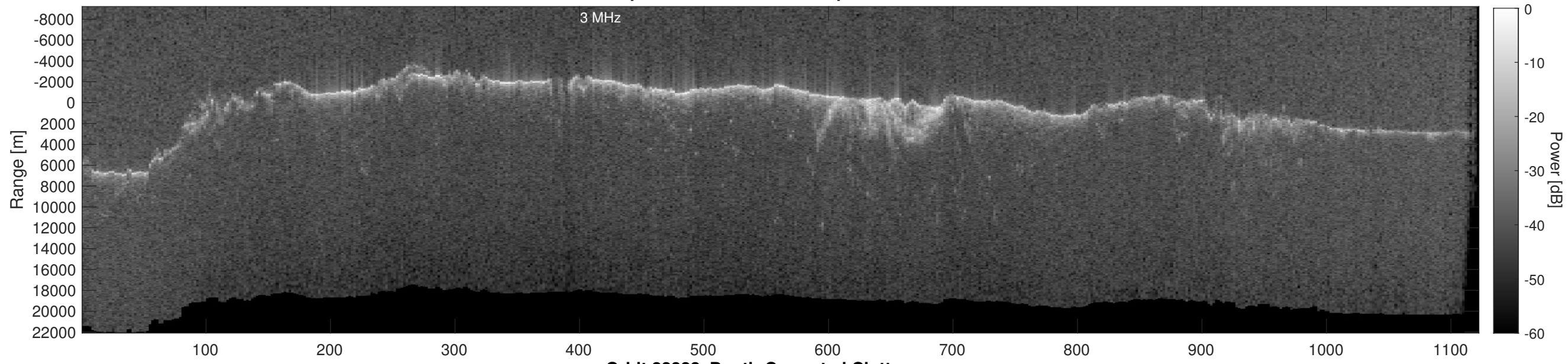
Orbit 22822, Depth-Corrected Cluttergram
