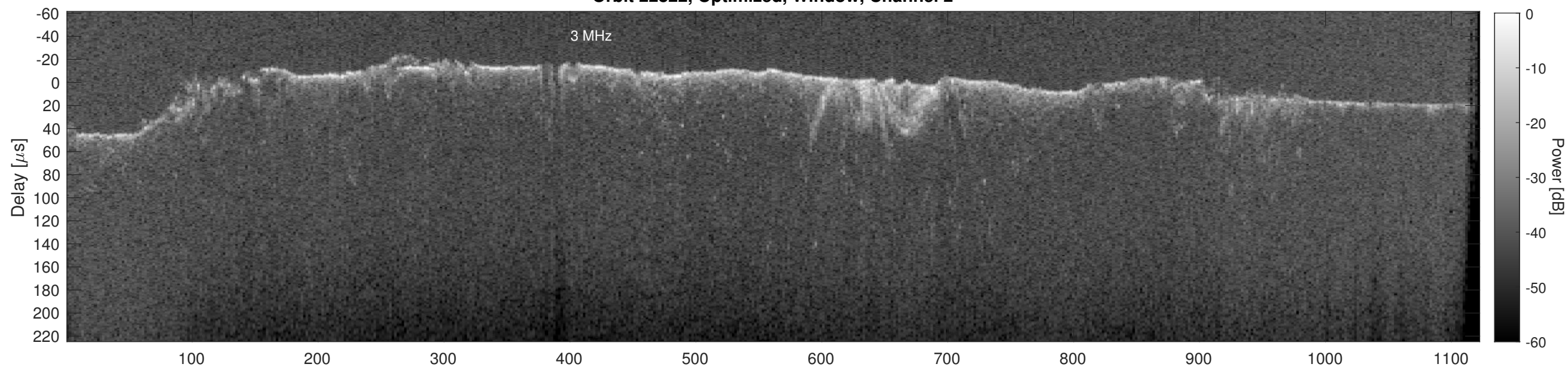
Orbit 22822, Cluttergram
