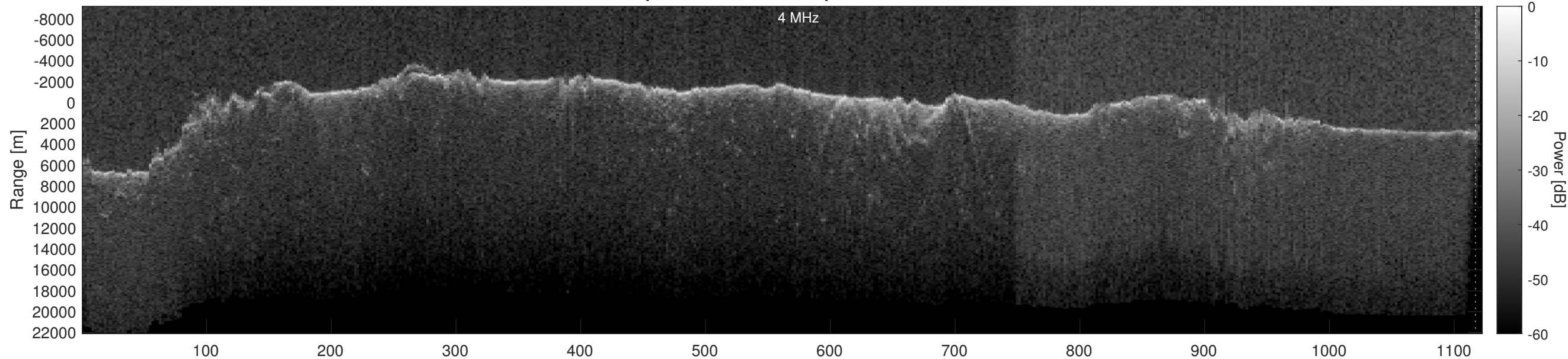
Orbit 22822, Optimized, Window, Depth-Corrected, Channel 2
