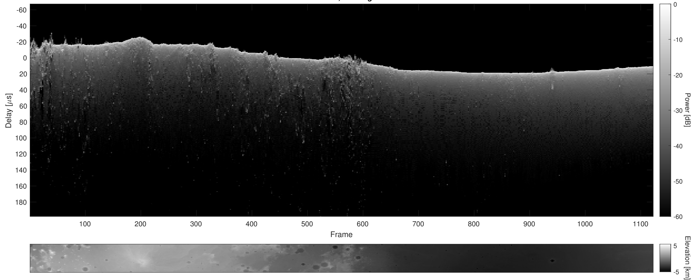
Orbit 22825, Cluttergram
