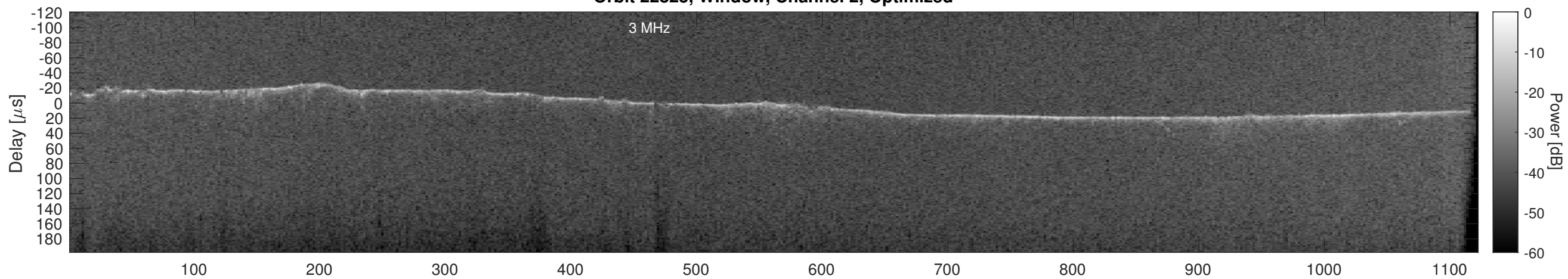
Orbit 22825, Cluttergram
