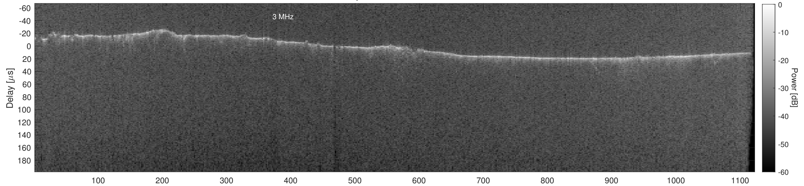
Orbit 22825, Cluttergram
