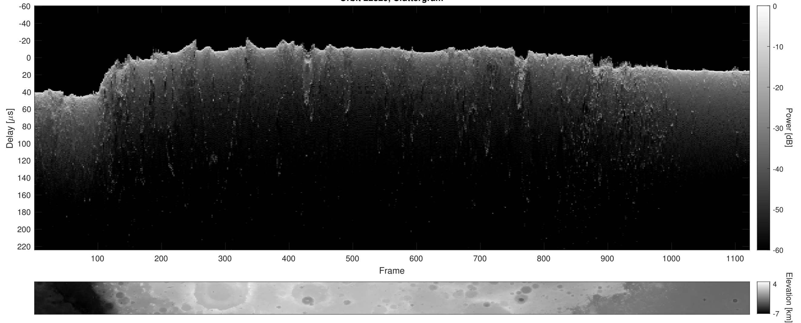
Orbit 22829, Cluttergram
