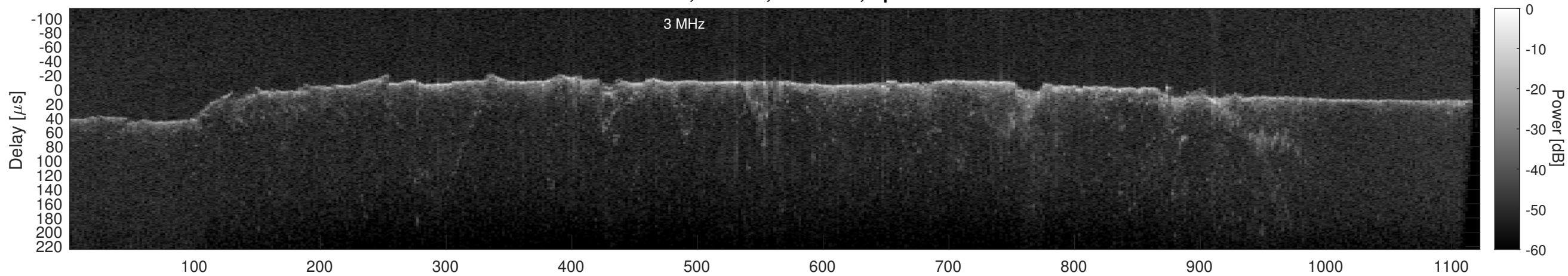
Orbit 22829, Cluttergram
