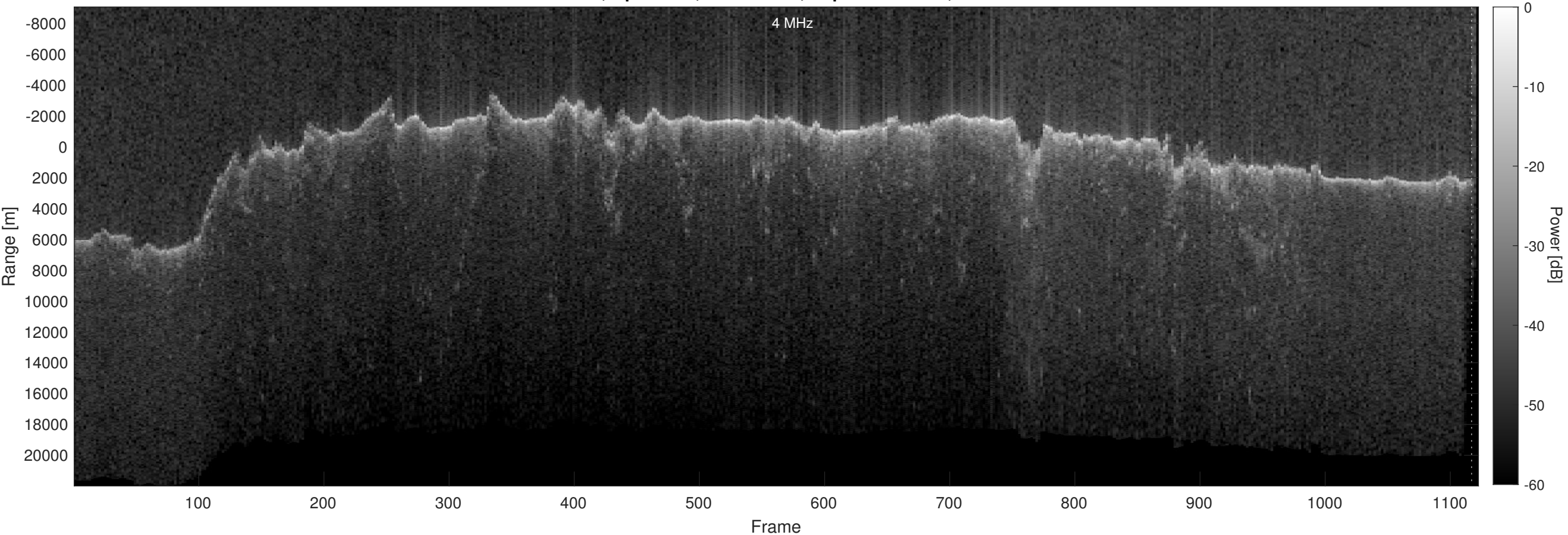
Orbit 22829, Optimized, No Window, Depth-Corrected, Channel 2
