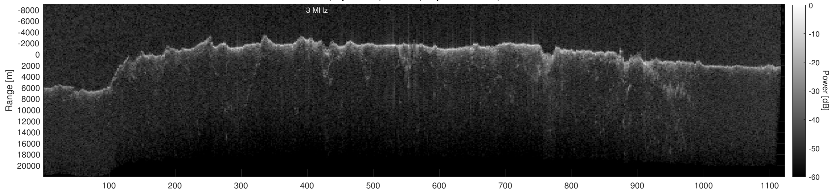
Orbit 22829, Depth-Corrected Cluttergram
