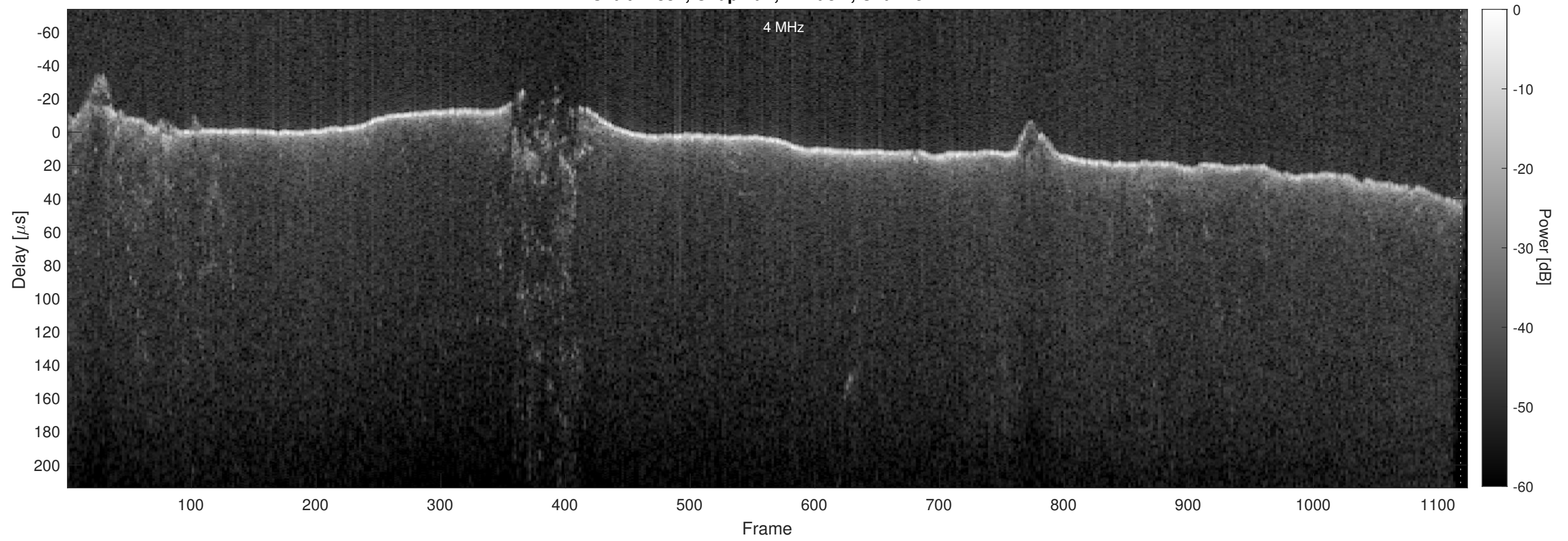
Orbit 22834, Chapman, Window, Channel 2
