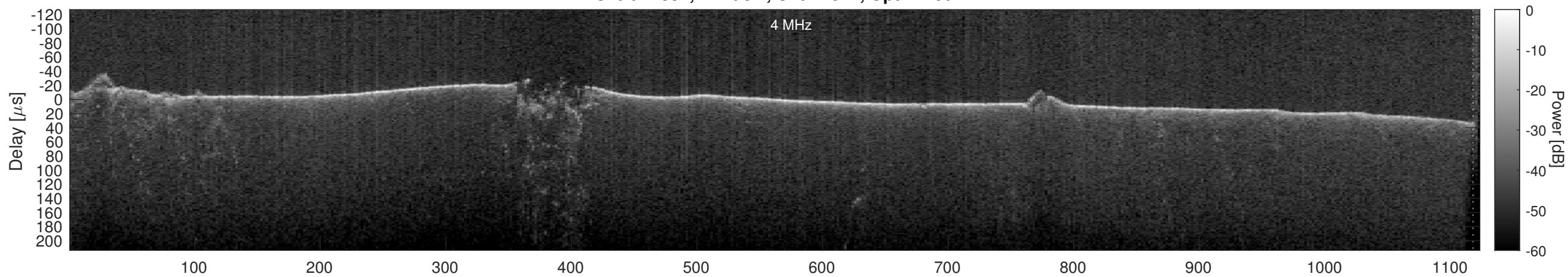
Orbit 22834, Cluttergram
