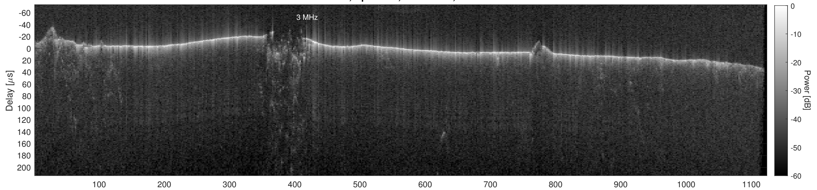
Orbit 22834, Cluttergram
