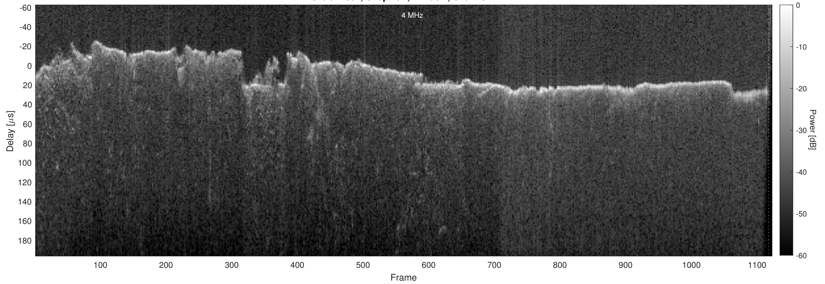
Orbit 22837, Chapman, Window, Channel 2
