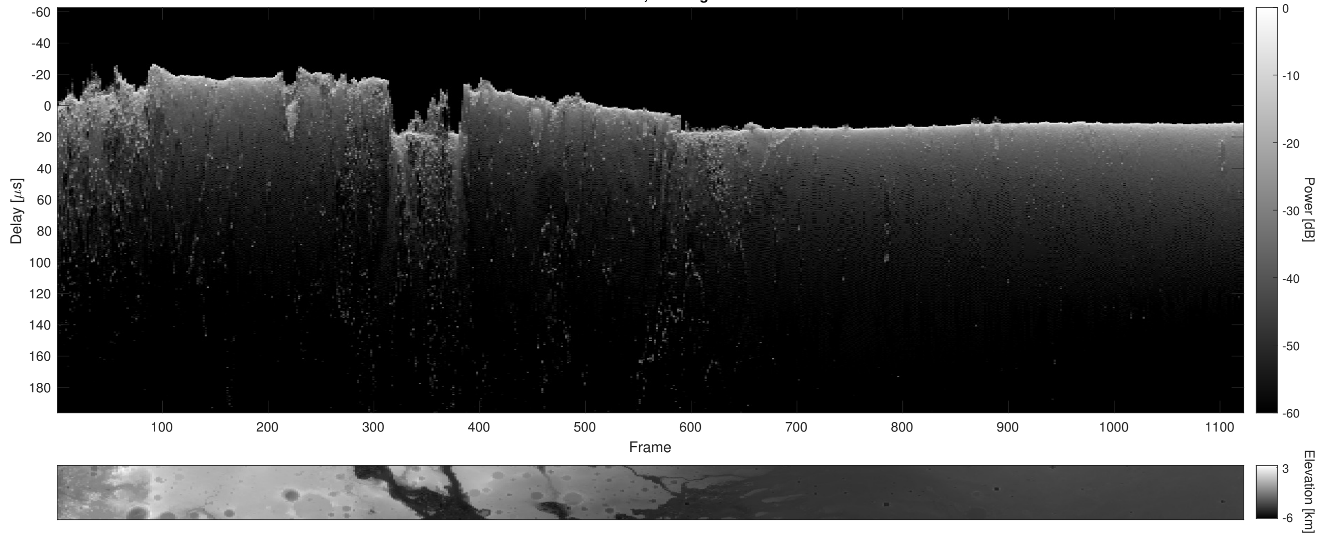
Orbit 22837, Cluttergram
