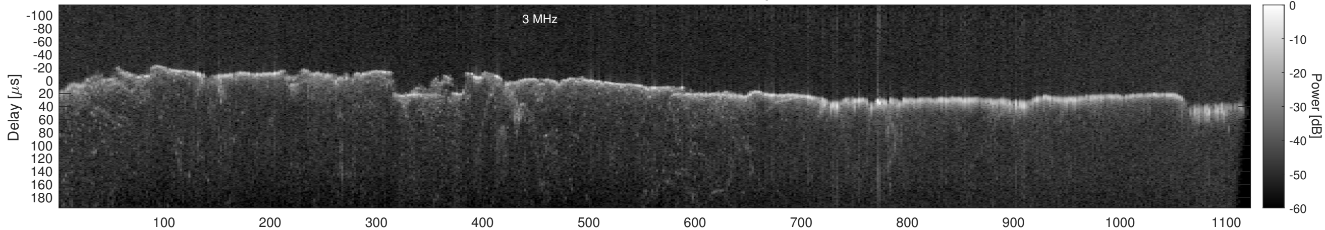
Orbit 22837, Window, Channel 2, Optimized
