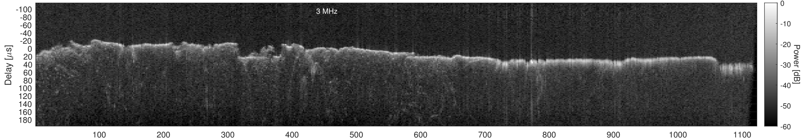
Orbit 22837, Window, Channel 2, Chapman
