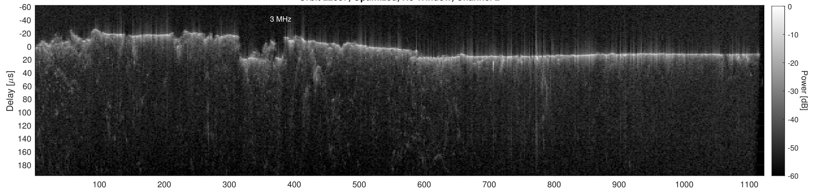
Orbit 22837, Cluttergram
