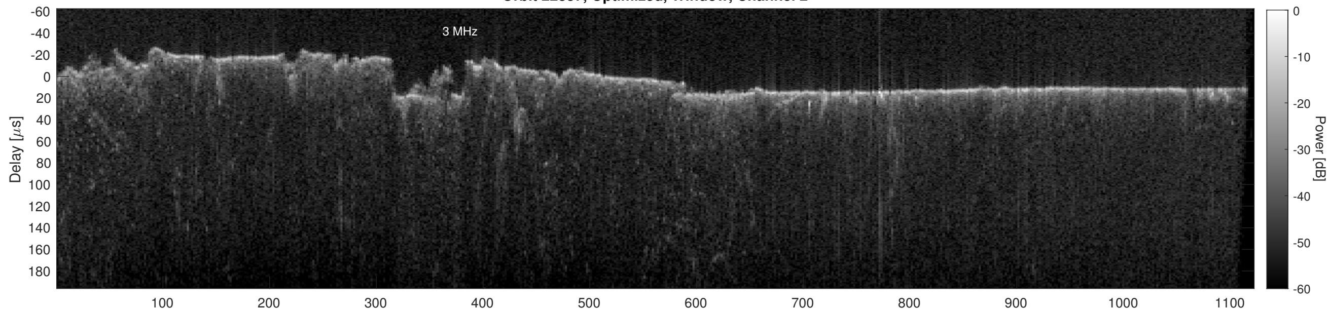
Orbit 22837, Cluttergram
