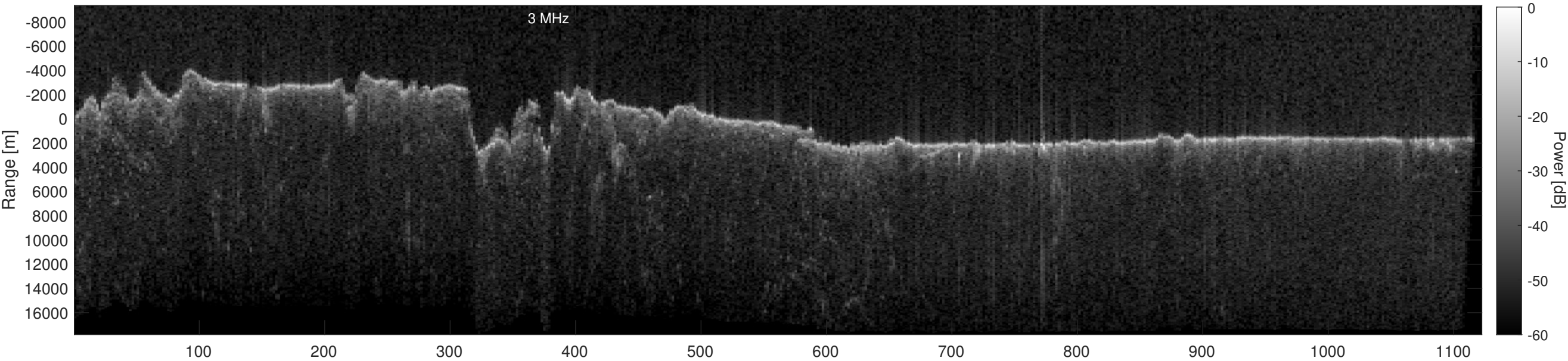
Orbit 22837, Depth-Corrected Cluttergram
