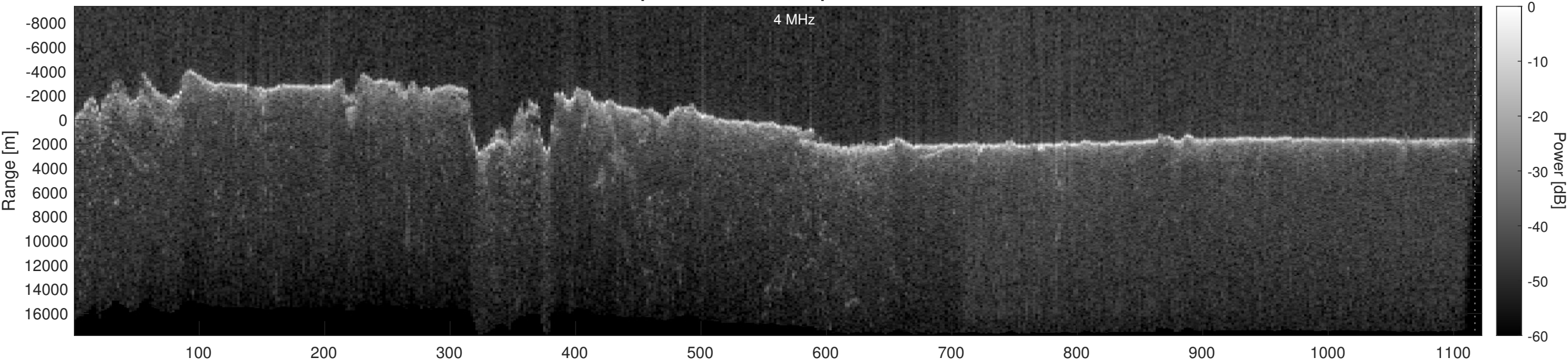
Orbit 22837, Optimized, Window, Depth-Corrected, Channel 2
