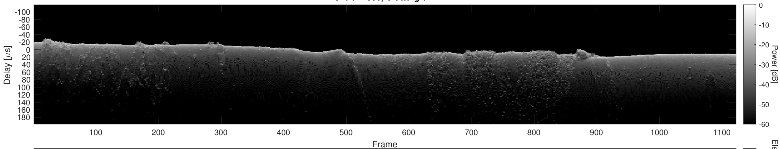
Orbit 22838, Cluttergram
