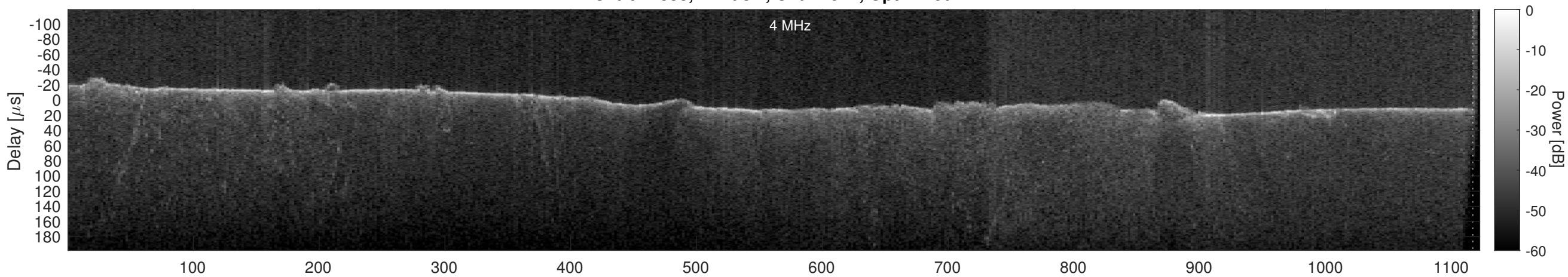
Orbit 22838, Cluttergram
