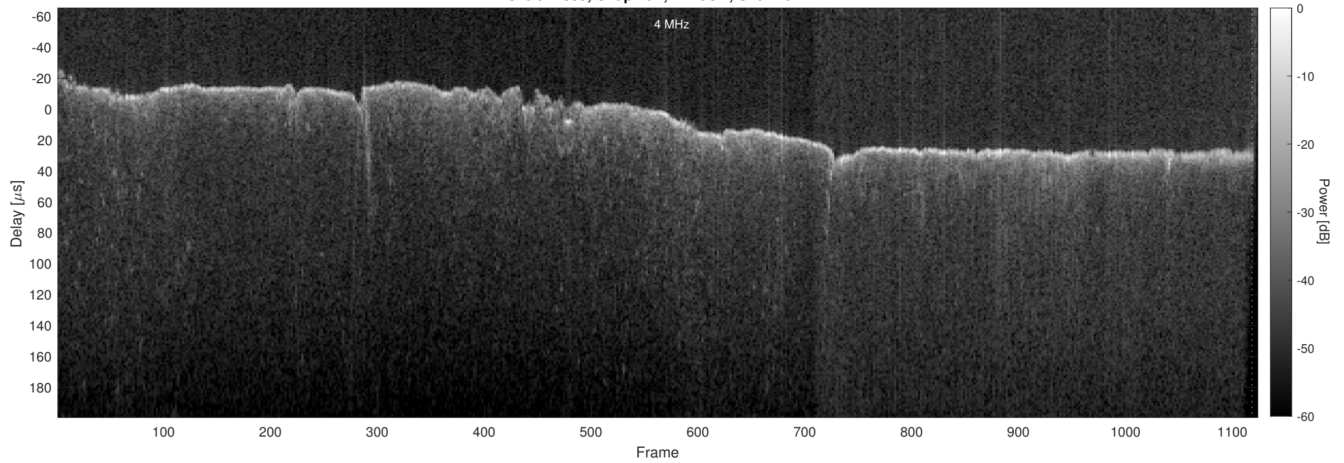
Orbit 22839, Chapman, Window, Channel 2
