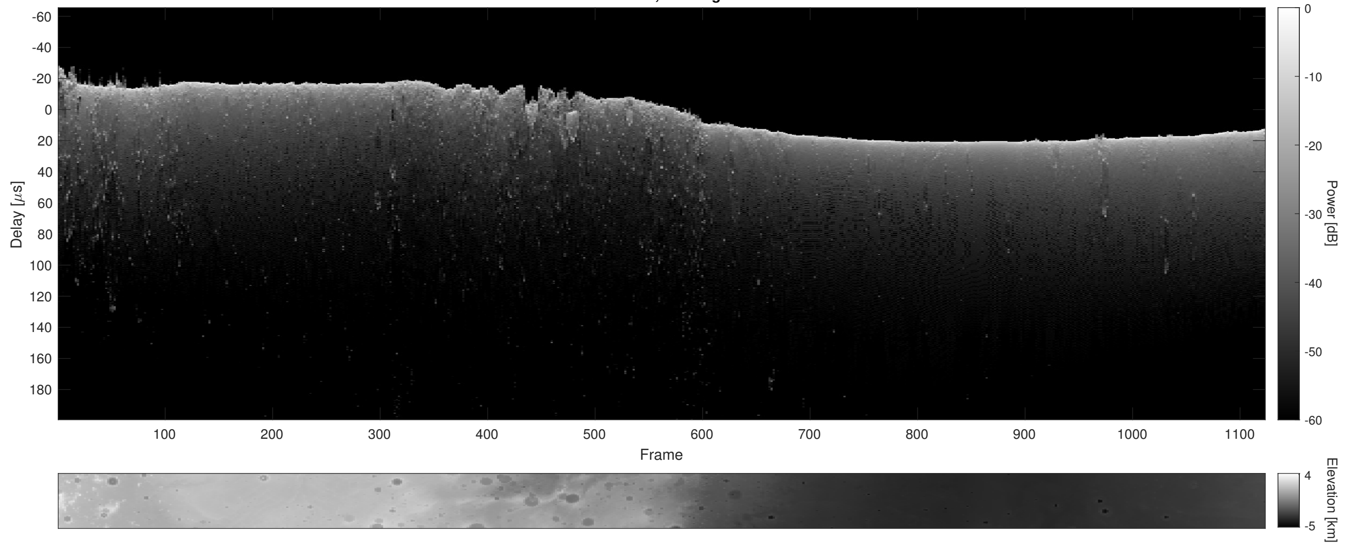
Orbit 22839, Cluttergram
