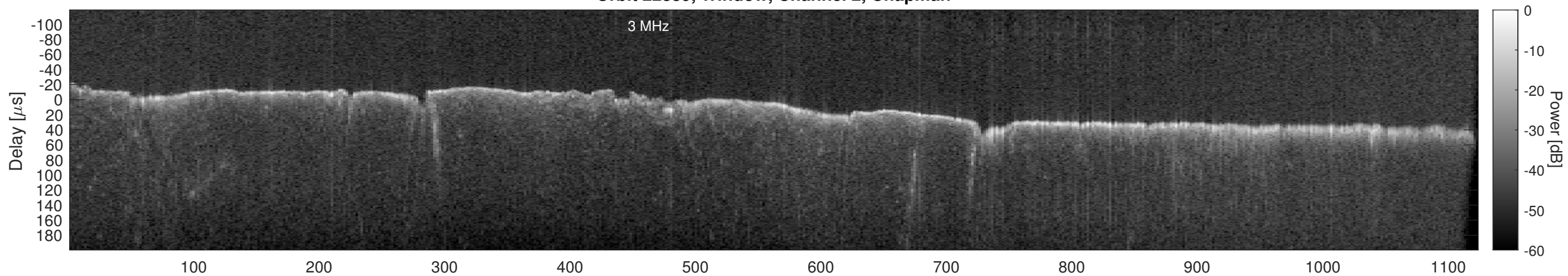
Orbit 22839, Window, Channel 2, Optimized
