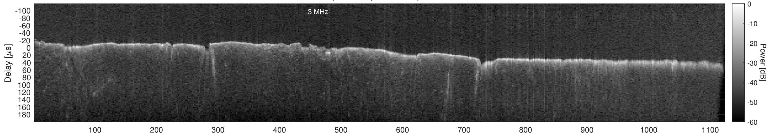
Orbit 22839, Window, Channel 2, Chapman
