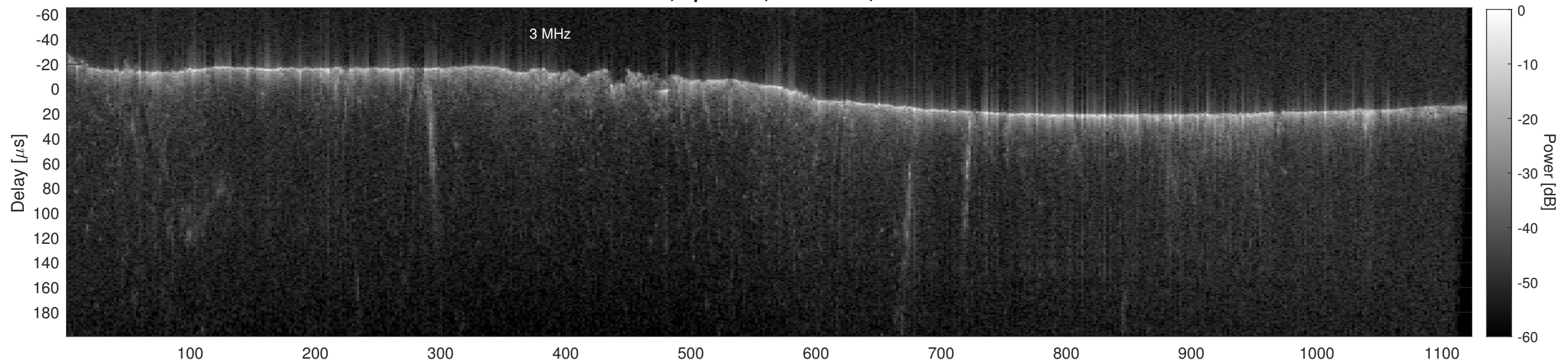
Orbit 22839, Cluttergram
