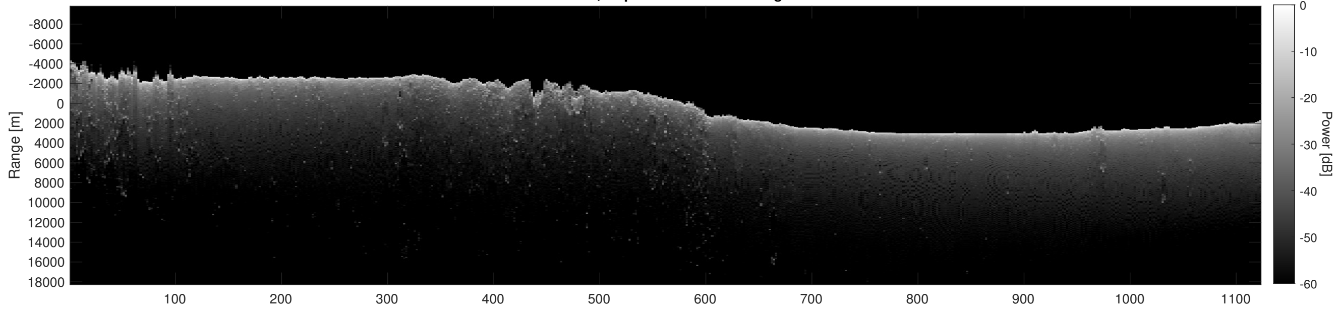
Orbit 22839, Depth-Corrected Cluttergram
