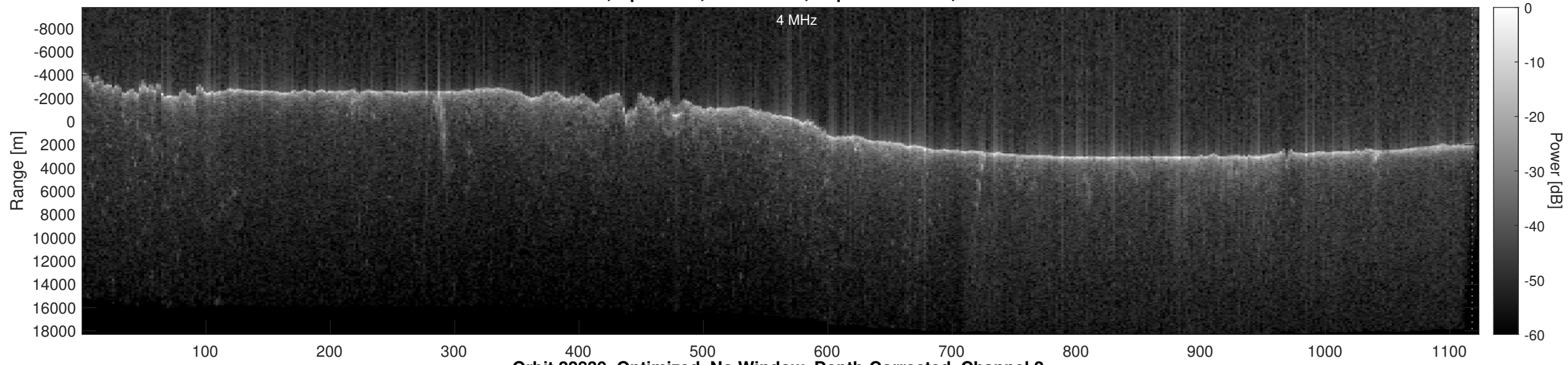
Orbit 22839, Optimized, No Window, Depth-Corrected, Channel 2
