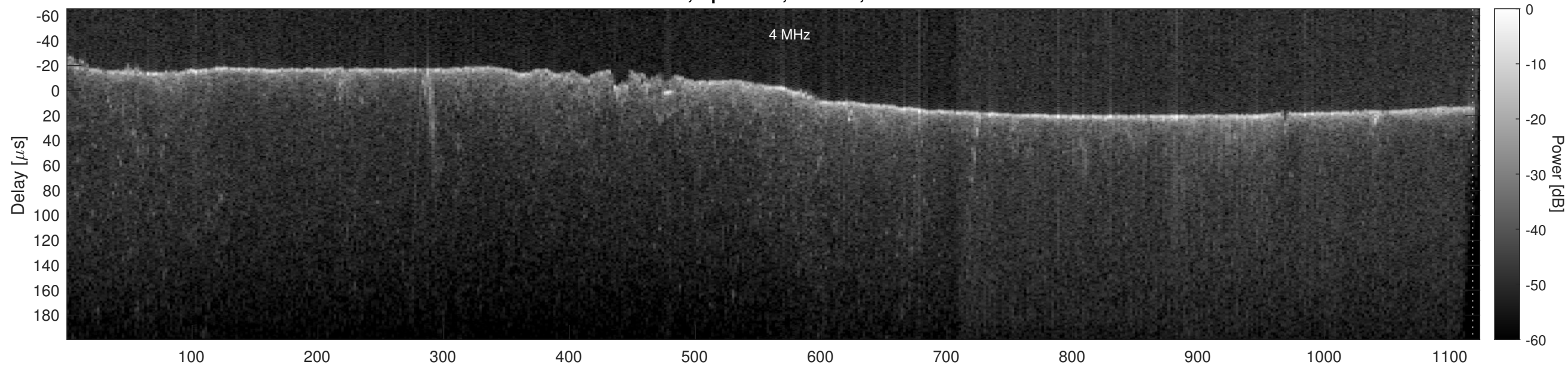
Orbit 22839, Optimized, Window, Channel 2
