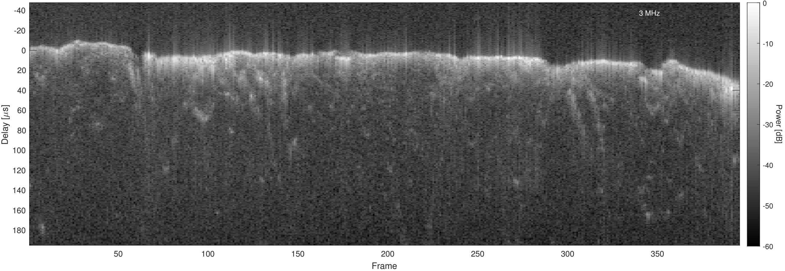
Orbit 22840, Chapman, No Window, Channel 2
