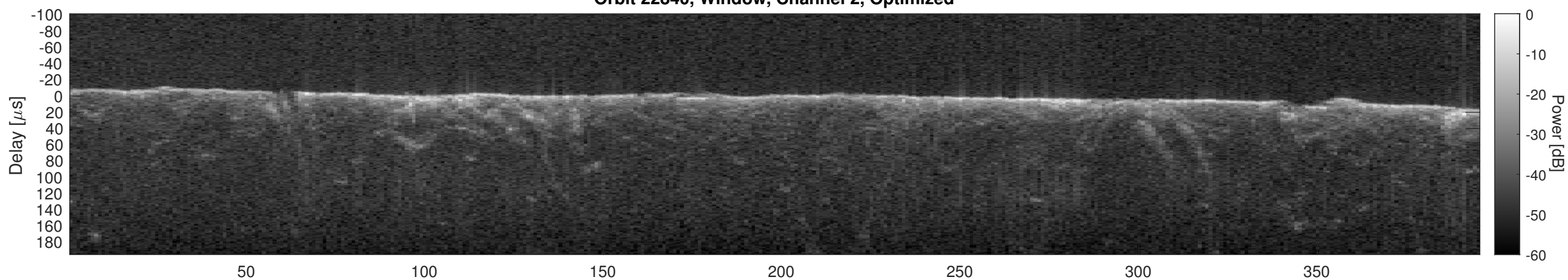
Orbit 22840, Cluttergram
