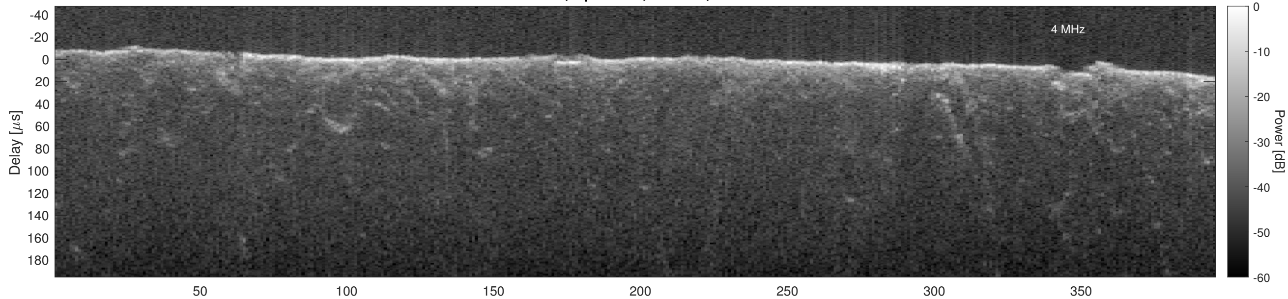
Orbit 22840, Optimized, Window, Channel 2
