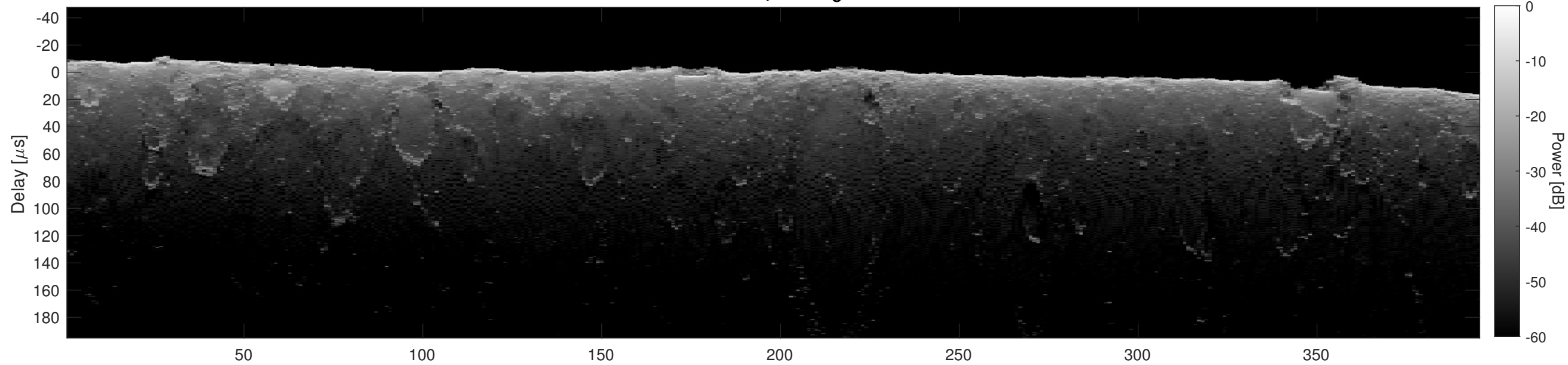
Orbit 22840, Cluttergram
