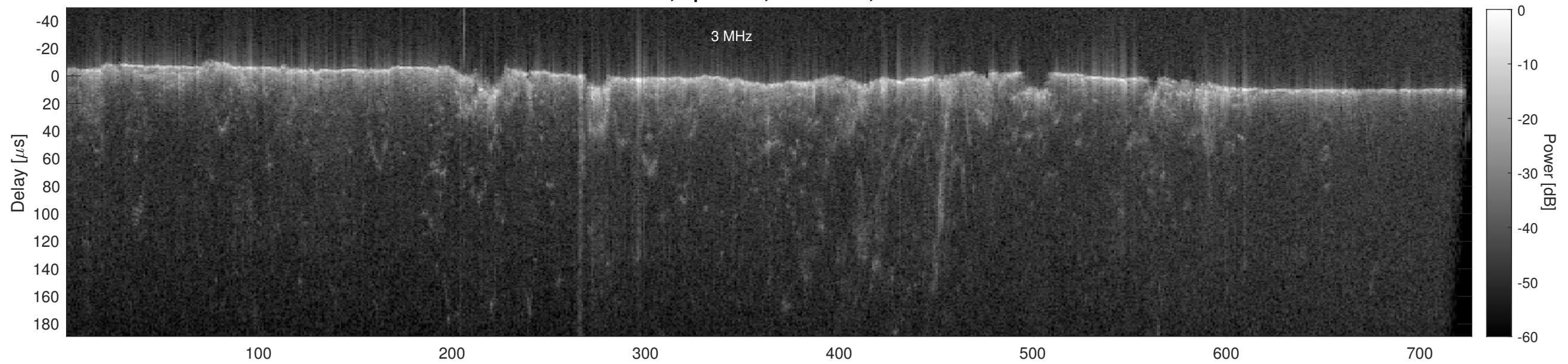
Orbit 22842, Cluttergram
