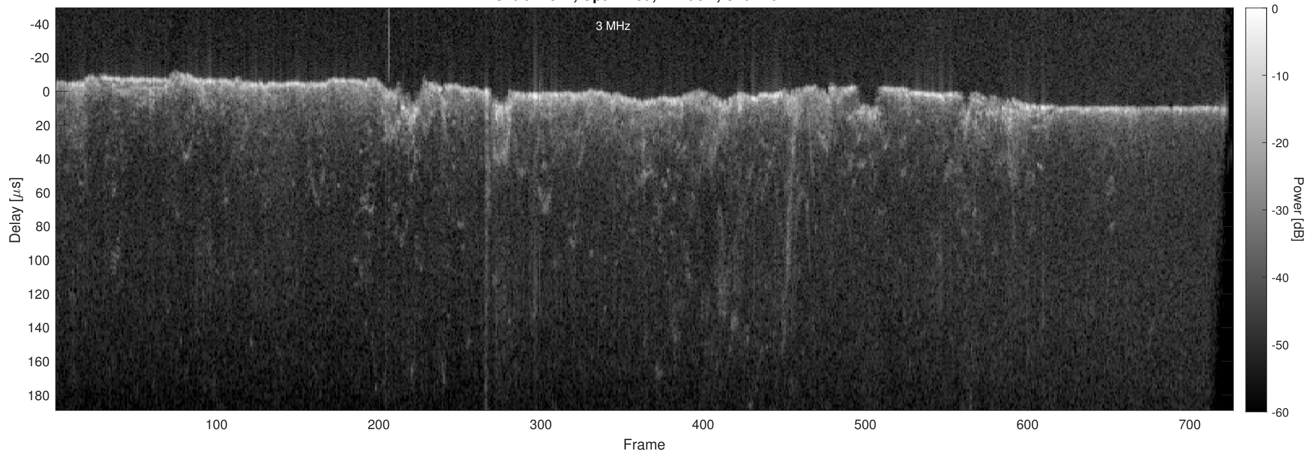
Orbit 22842, Optimized, Window, Channel 2
