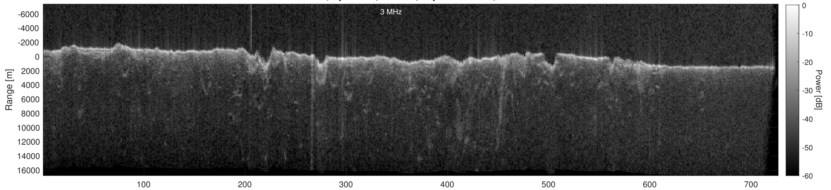
Orbit 22842, Depth-Corrected Cluttergram
