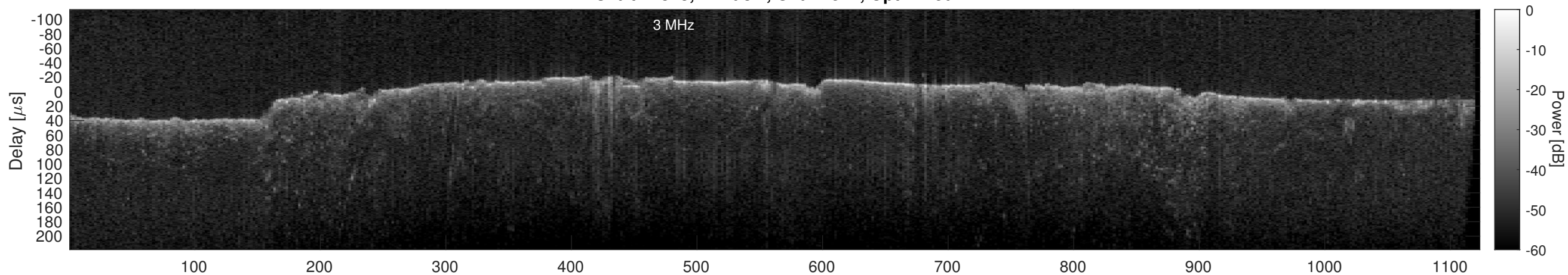
Orbit 22843, Cluttergram
