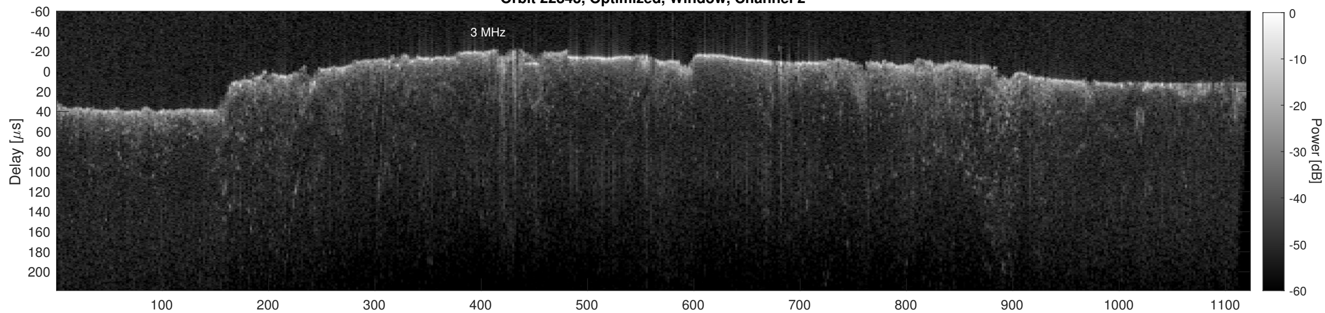
Orbit 22843, Cluttergram
