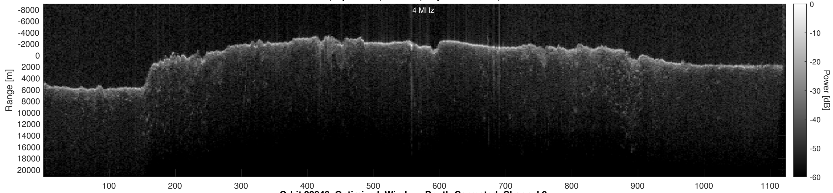
Orbit 22843, Optimized, Window, Depth-Corrected, Channel 2
