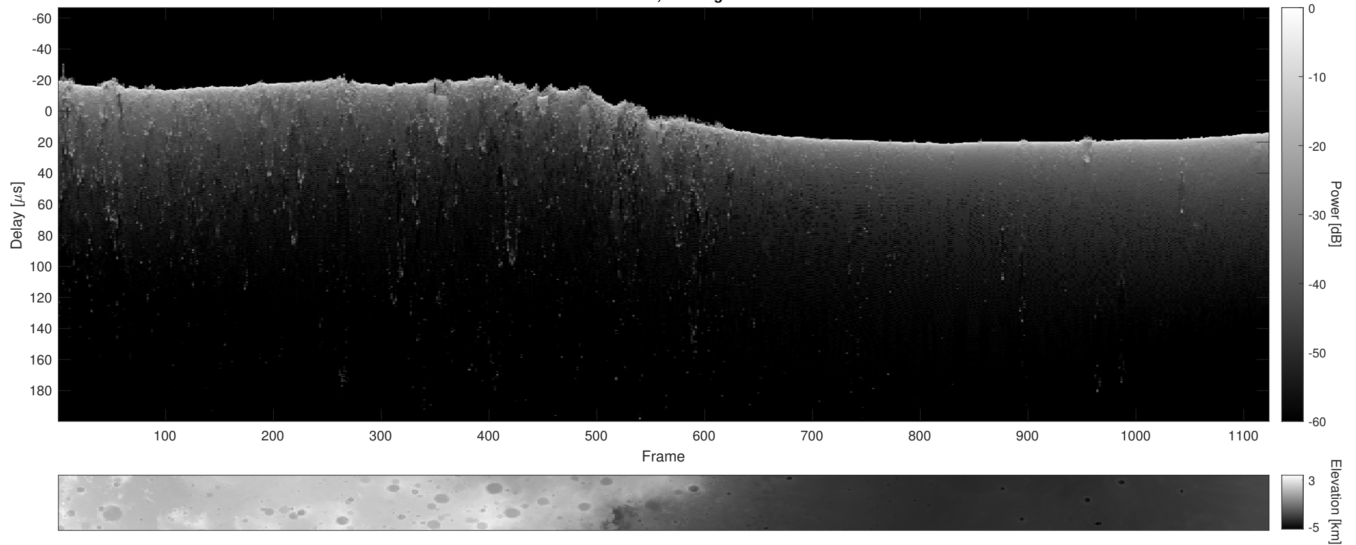
Orbit 22846, Cluttergram
