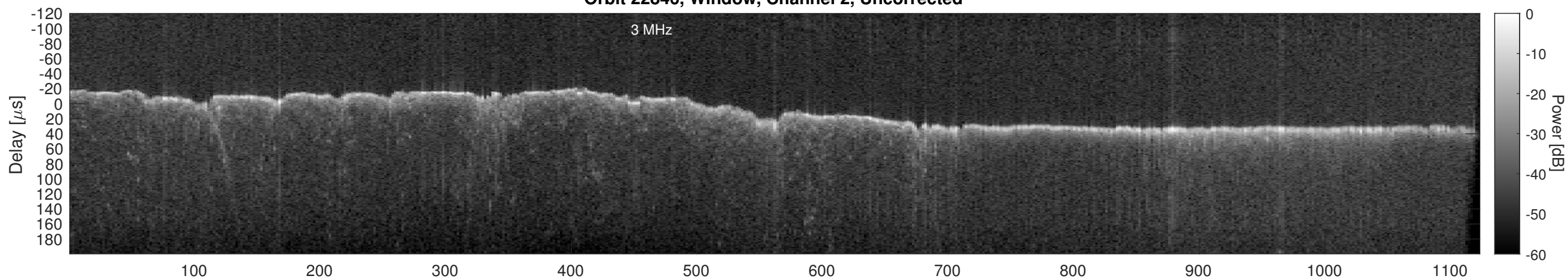
Orbit 22846, Window, Channel 2, Chapman
