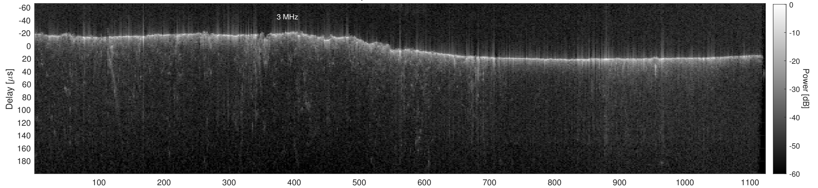
Orbit 22846, Cluttergram
